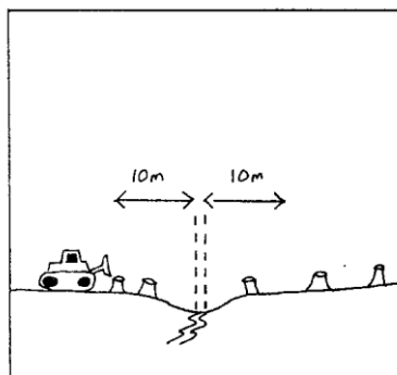
Standard Class 4 machinery exclusion zone (MEZ)
